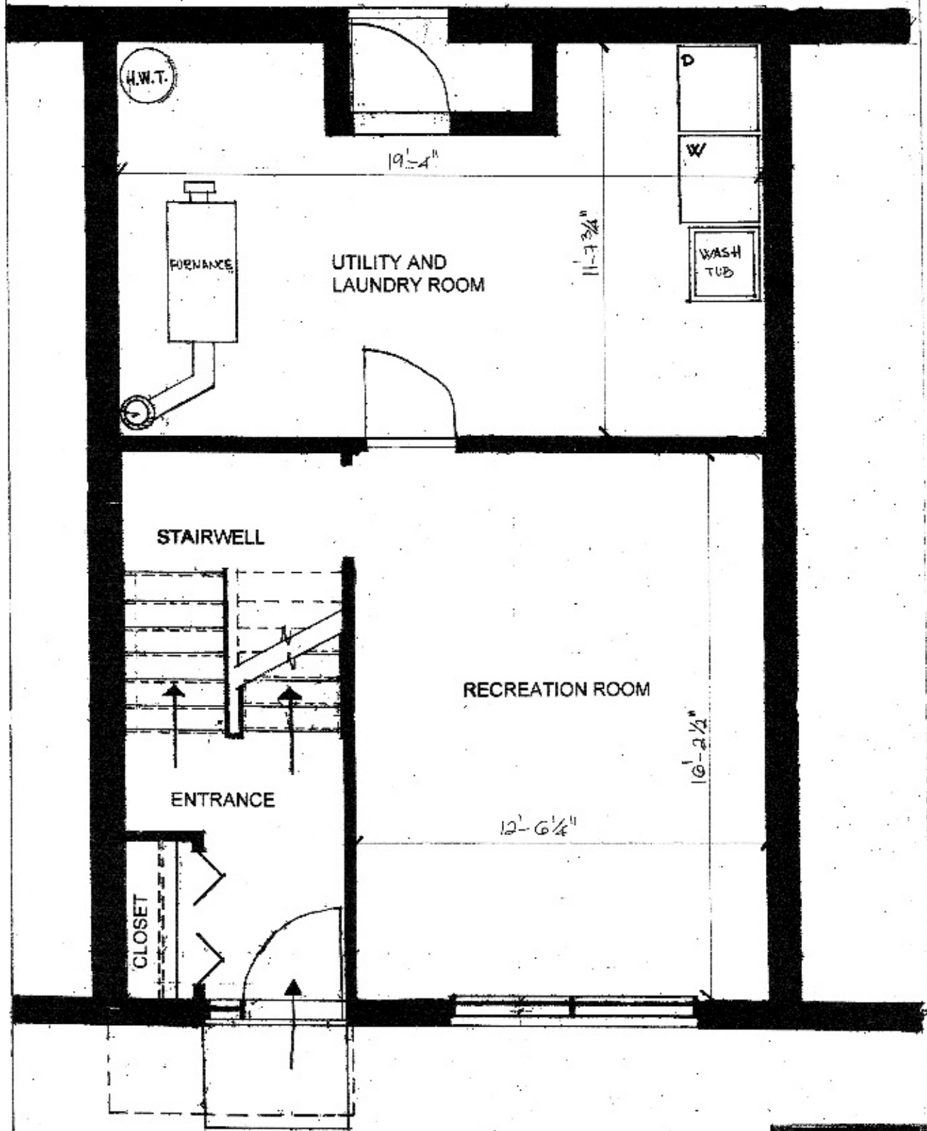
COSTELLO 3 BEDROOM - BASEMENT PLAN SCALE: 1/4" = 1'-0"
