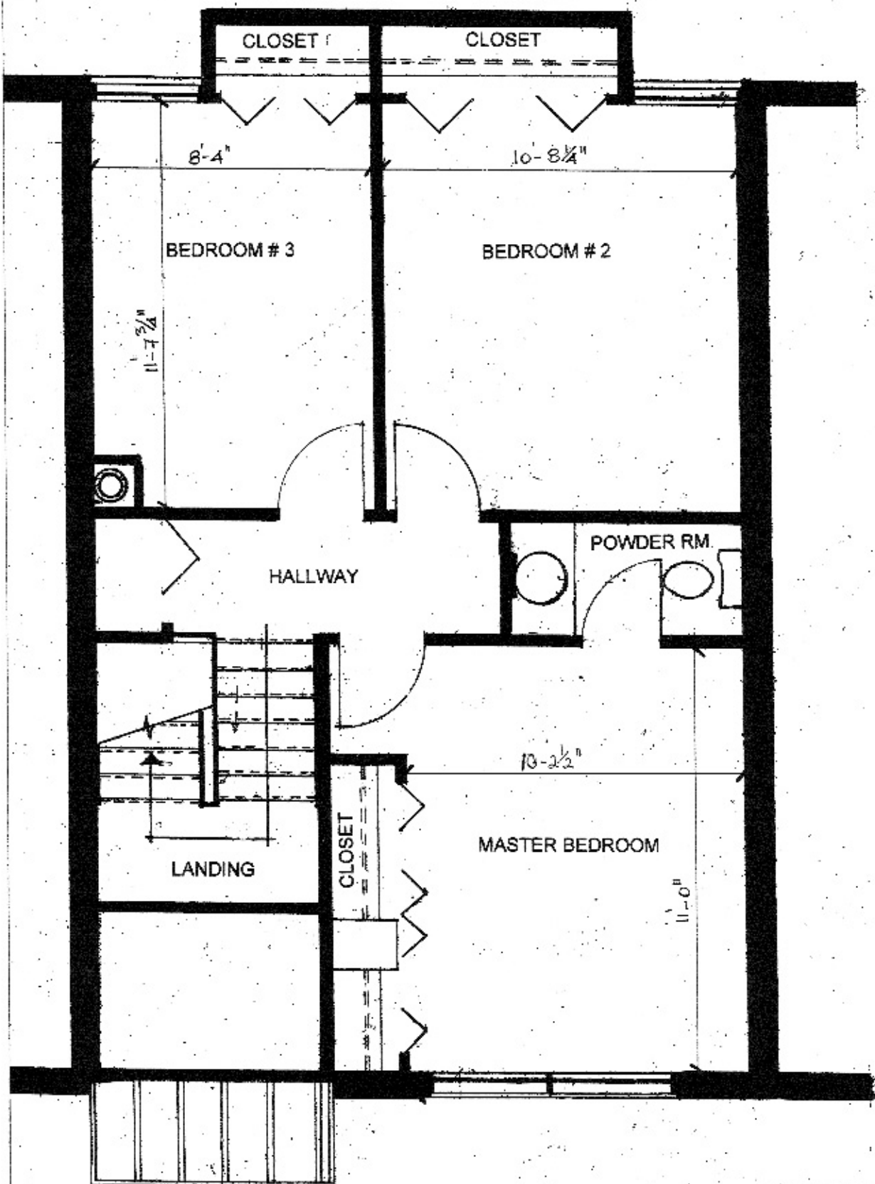
COSTELLO 3 BEDROOM - SECOND FLOOR PLAN SCALE: 1/4" = 1'-0"
