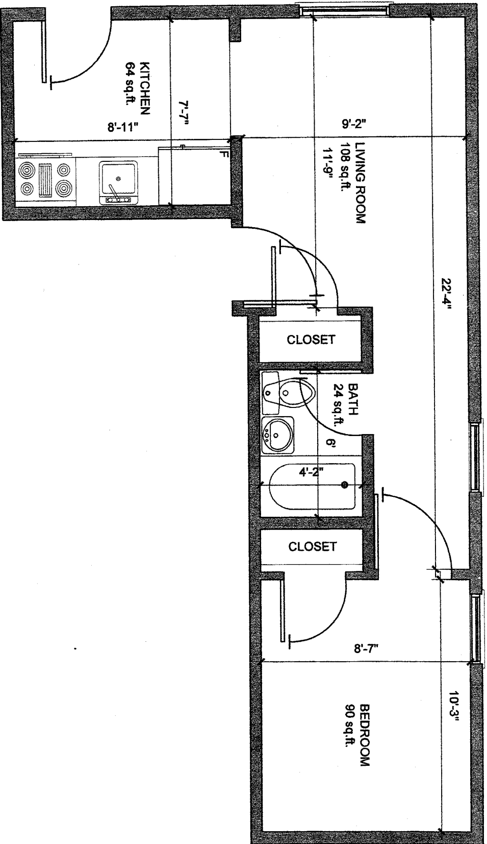
PALAZZI PLACE 1 BEDROOM PLAN LAYOUT SCALE: 1/4" = 1'-0"
